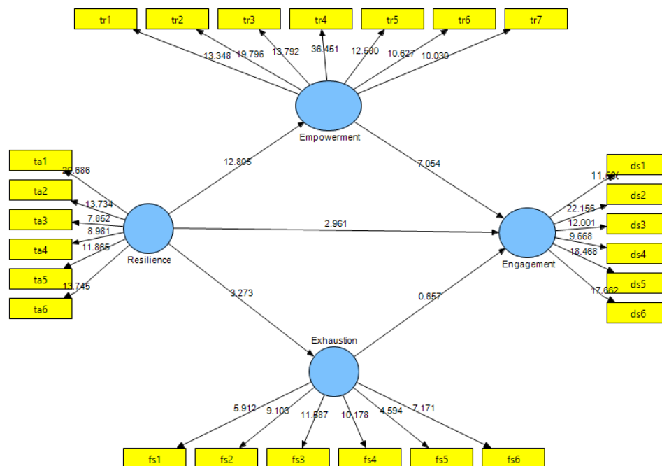
Fig. 2. T- Statistics
